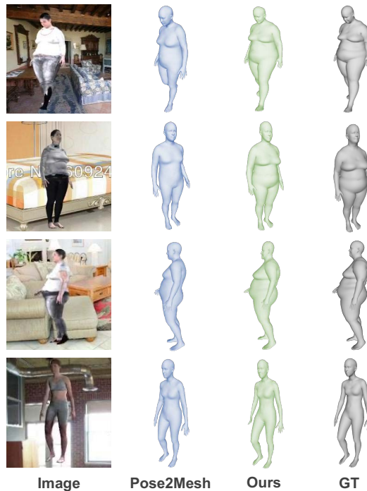
Figure 1. Mesh estimation results on four examples with different body shapes. Pose2Mesh [7] which uses 3D skeletons as the intermediate representation fails to predict accurate shapes. Our virtual marker-based method obtains accurate estimates.
